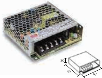
LED-TRRS/12/75 (4.2A)
