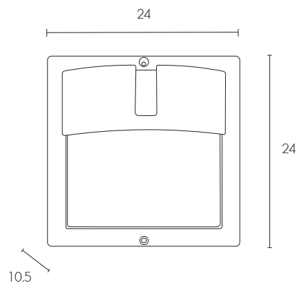
WM-660 E27 Aluminium + PC 1,440.-
