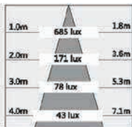
OPL-DHM14/40°-14W-4000K-1200LM
