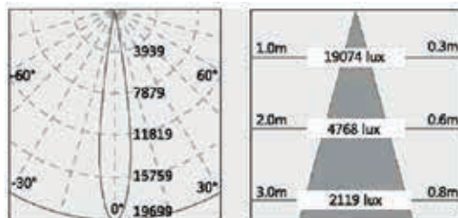
OPL-ROUND-LA-30W-WM-24°-3000K
