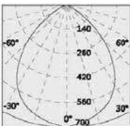
OPL-DHM14/40°-14W-4000K-1200LM
