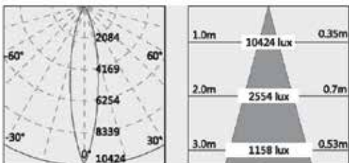
OPL-ROUND-LA-30W-WM-40°-3000K
