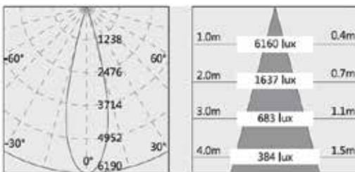
OPL-ROUND-MA-16-WM-24°-3000K
