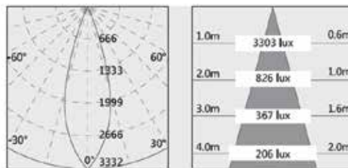
OPL-ROUND-MA-16-WM-40°-3000K
