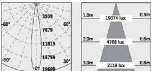
OPL-ROUND-LA-30W-WM-24°-3000K
