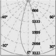
OPL-ROUND-MA -16-MW-40° -3000K
