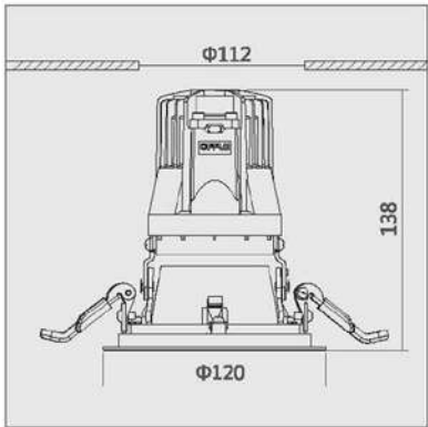
OPL-ROUND-MA -16-MW-24° -3000K
