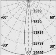
OPL-ROUND-MA -16-MW-24° -3000K
