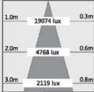
OPL-ROUND-MA -16-MW-24° -3000K
