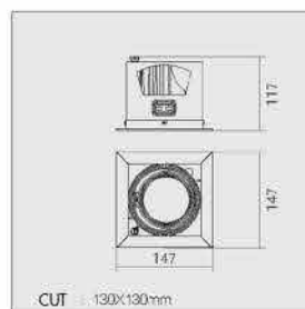
OPL-MATRIX-L1 / 30 OPL-MATRIX-L1 / 40 LED 30W (3000K, 4000K)
