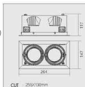
OPL-MATRIX-L2 / 30 OPL-MATRIX-L2 / 40 LED 30W x 2 (3000K, 4000K)
