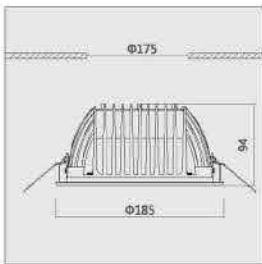
OPL-DHM14/30 OPL-DHM14/40 OPL-DHM14/57 LED 14W (3000K,4000K, 5700K)
