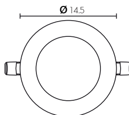
LED-PN009E/30/LTO LED-PN009E/40/LTO LED-PN009E/60/LTO
