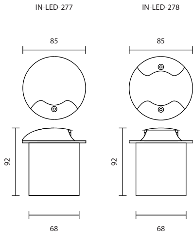
IN-LED-277 LED 2W 220V 3000K 1,900.-
