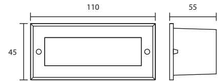
STEP-1511/S/LED E27 LED 220V 1W 800.-
