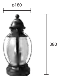
O-8200S E27 GENIE 18W E27 LED A60 7W/9W 1,100.-
