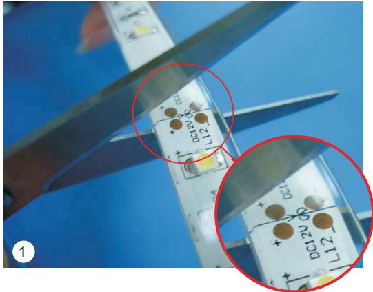
1. Please cut the LED strip at the cutting line.
