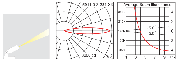
QR-CB51GU53 Par20 10°
