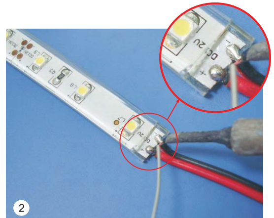
2. Rejoin the cables to the strip by soldering, please do not reverse the polarity.
